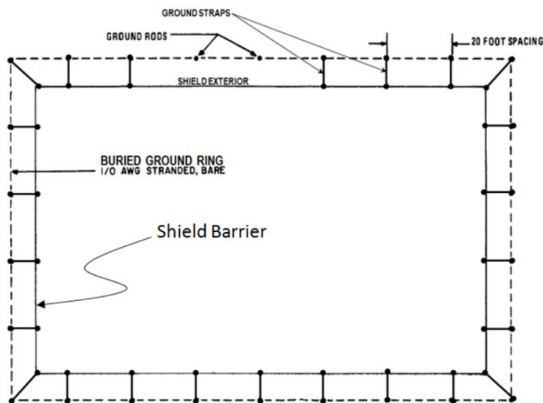
Figure 34. Shield barrier earth electrode system
