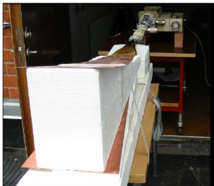
Figure 18. Laboratory hyperband pulse generator used in Russia
