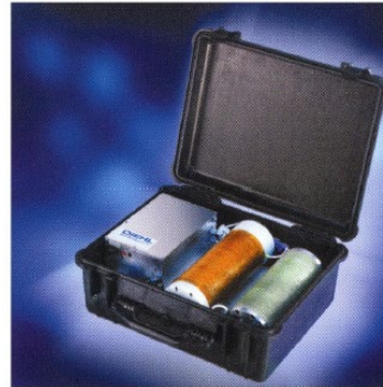
Figure 17. DIEHL Munitions damped sine IEMI generator
